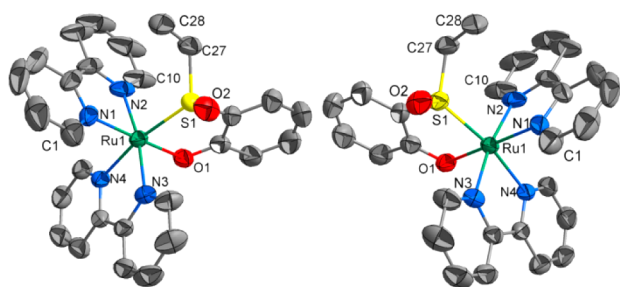
Figure 5. View of the structures of a pair of cations in rac - 2a (left, \Delta - R ; and right, \Lambda - S ). Selected bond angles (deg) and distances (Å): Ru1–O1 = 2.076(3), Ru1–S1 = 2.250(1), Ru1–N1 = 2.060(4), Ru1–N2 = 2.058(4), Ru1–N3 = 2.070(4), Ru1–N4 = 2.105(3), S1–O2 = 1.487(4), N4–Ru1–S1 = 168.5(1). ORTEP drawing with 50% probability thermal ellipsoids. 19
